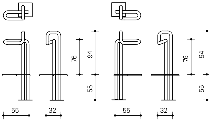
Type LS.2 Links
