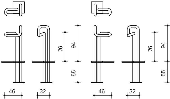
Type LS.1 Links
